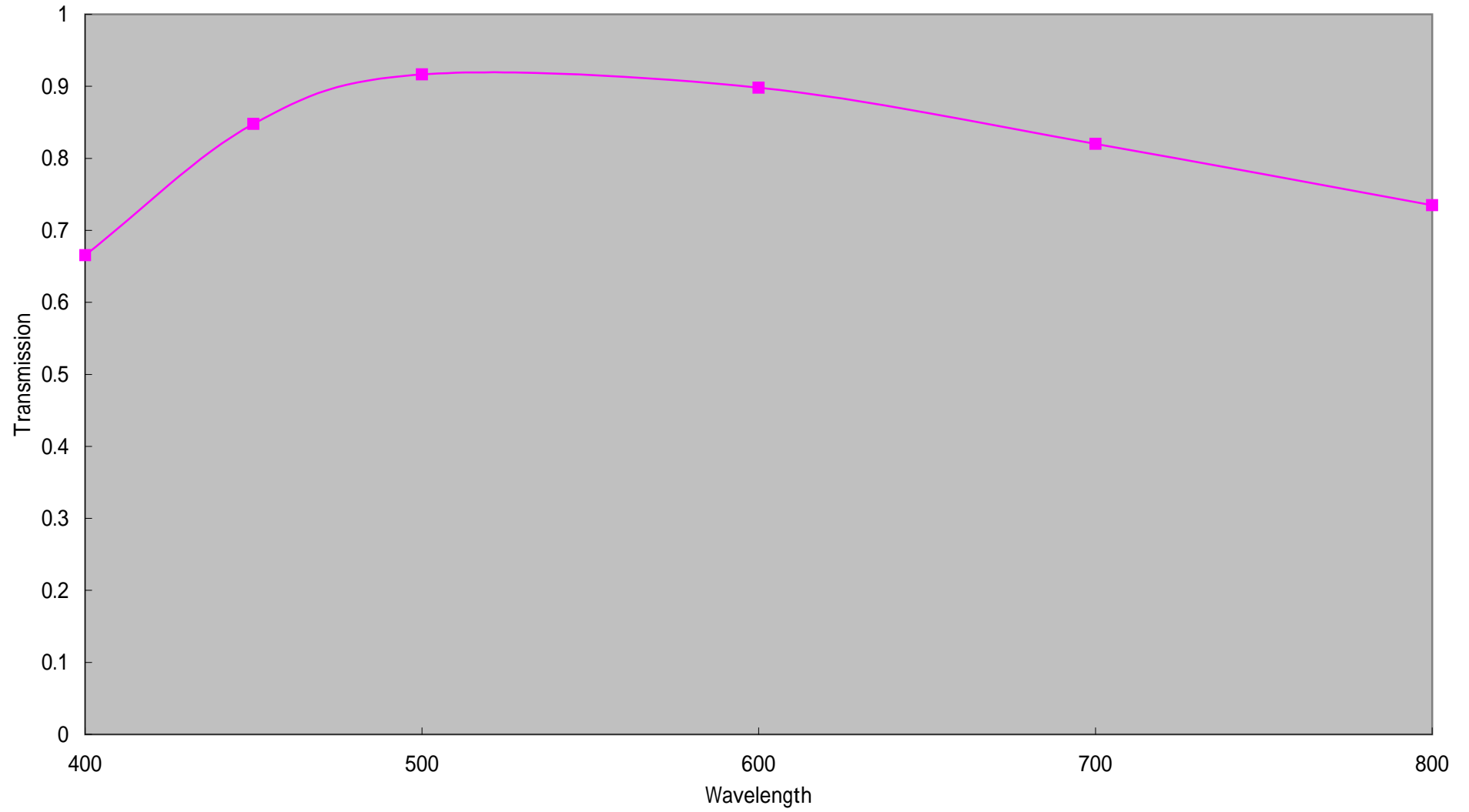
LM12NCL (604) Transmission
